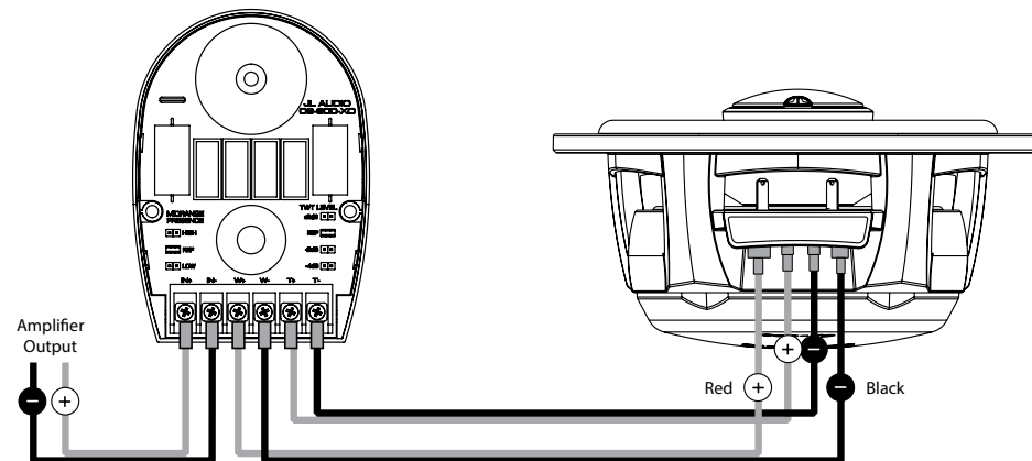
DIAGRAM B: Coaxial System Wiring
