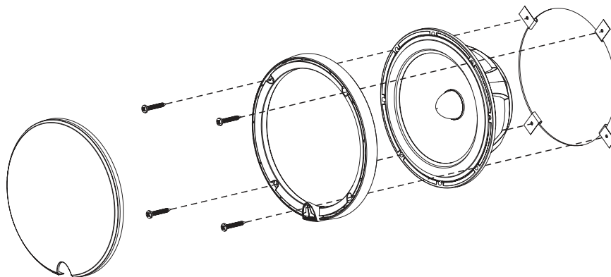
DIAGRAM J: Custom Location Woofer Installation
