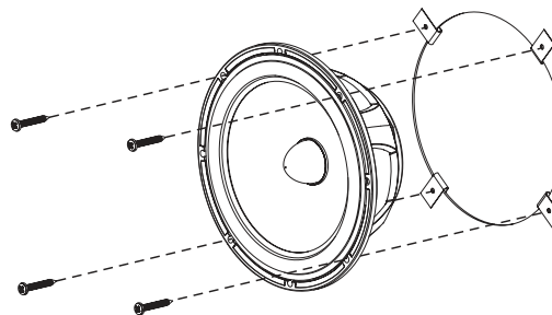
DIAGRAM I: Factory Location Woofer Installation
