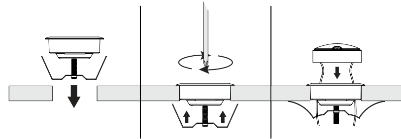
DIAGRAM K: Flush-Mount Tweeter Installation
