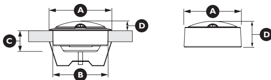
Tweeter Fixture Physical Dimensions
