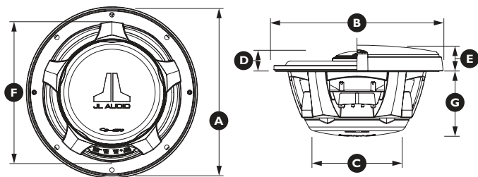
Woofer Physical Dimensions
