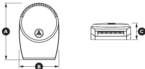
Crossover Network Physical Dimensions
