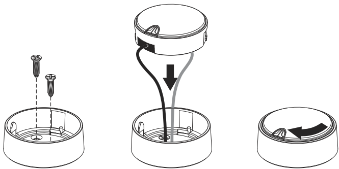
DIAGRAM L: Surface-Mount Tweeter Installation
