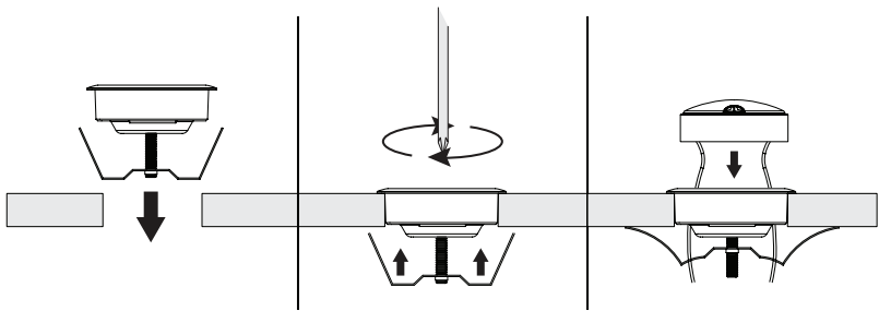
DIAGRAM K: Flush-Mount Tweeter Installation
