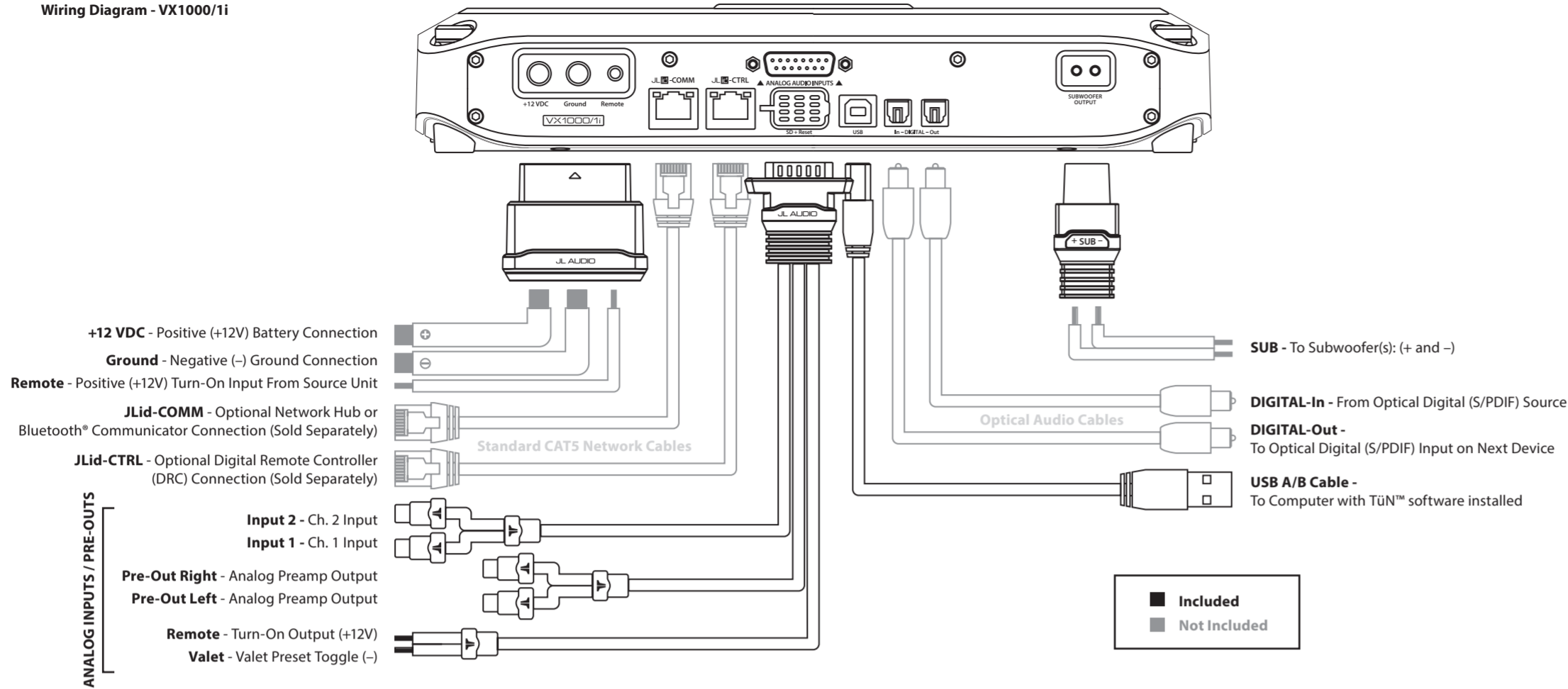
Wiring Diagram - VX1000/1i
