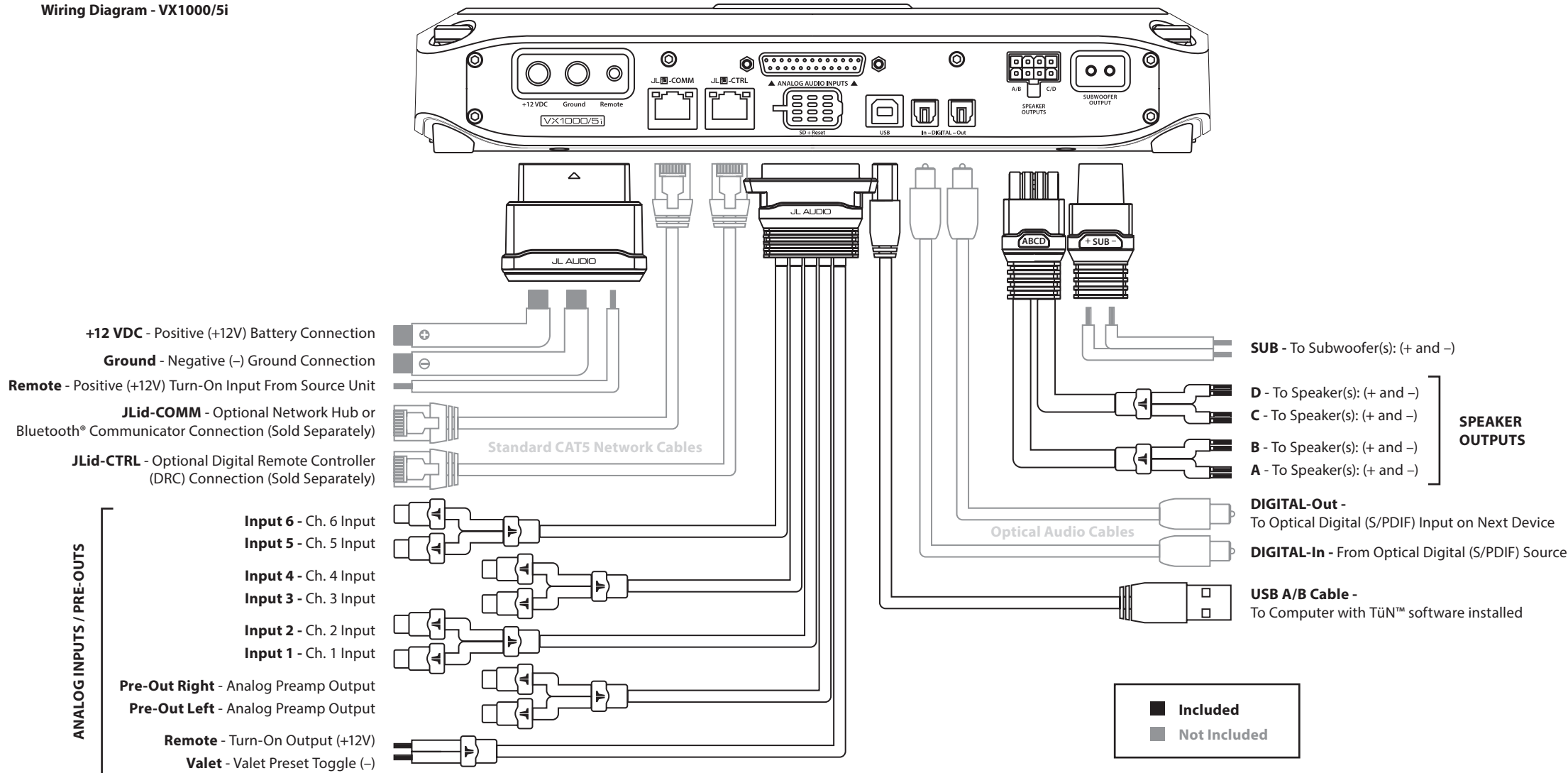
Wiring Diagram - VX1000/5i
