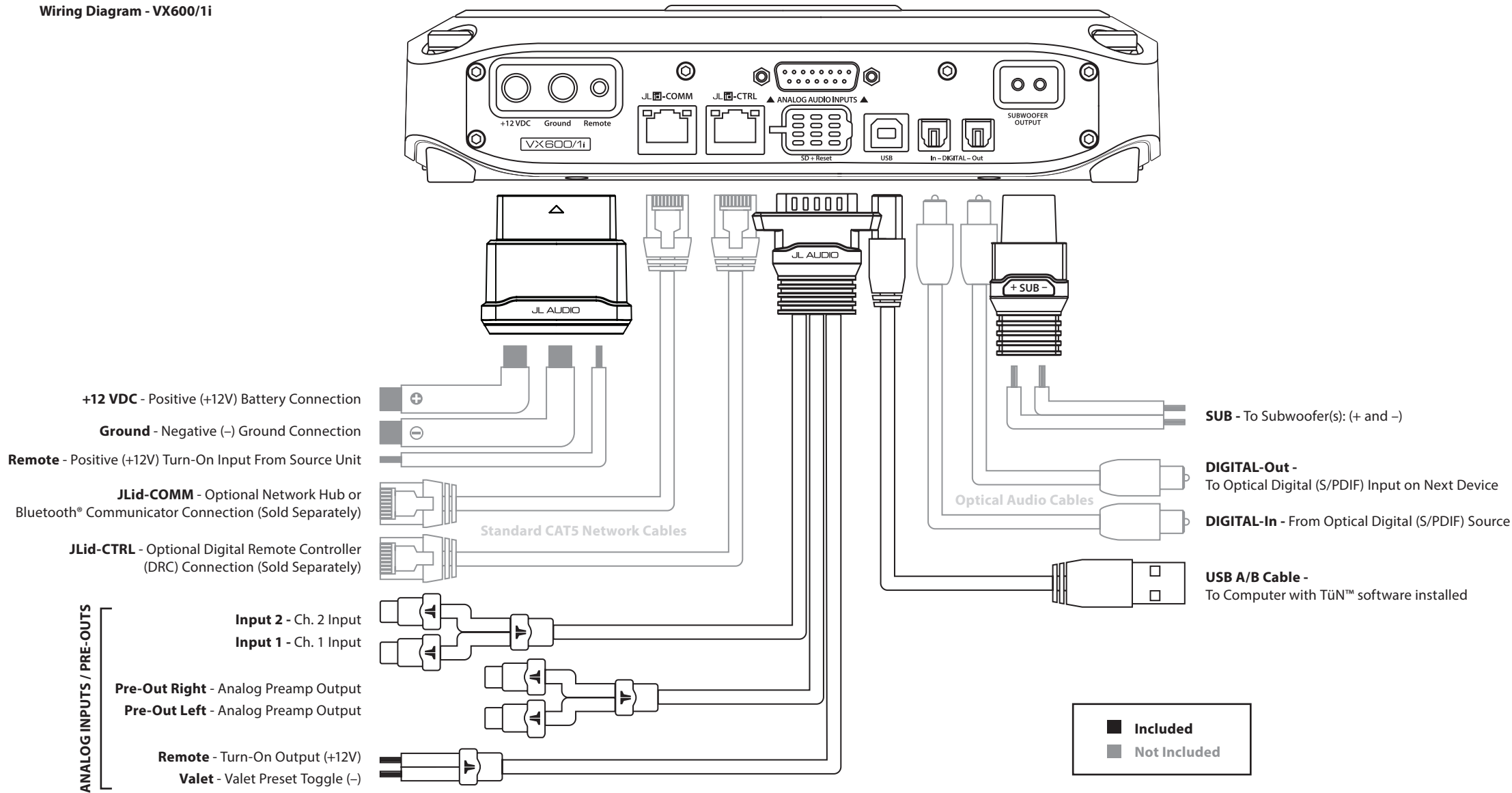
Wiring Diagram - VX600/1i
